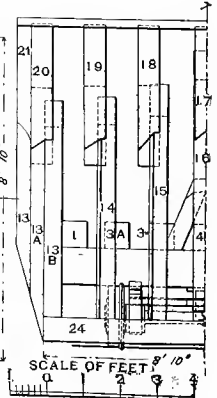
Fig. 413. Half Front End Elevation.
